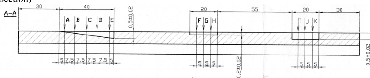
Figure 2.1 – Dimensions of specimens
