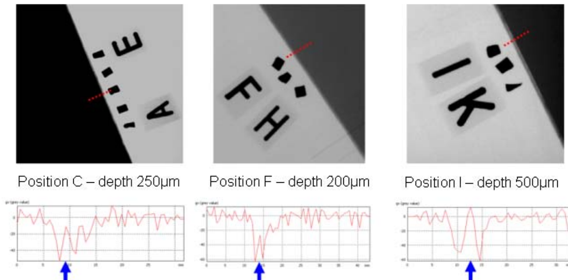
Figure 5.1 – The gray value profiles in place of the artificial flaw
