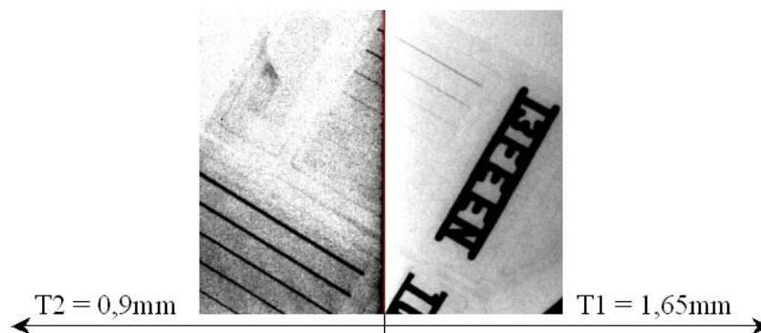
Figure 4.2 – Pixel line – IQI wire angle: approx. 30°, contrast adjusted for each thickness separately
