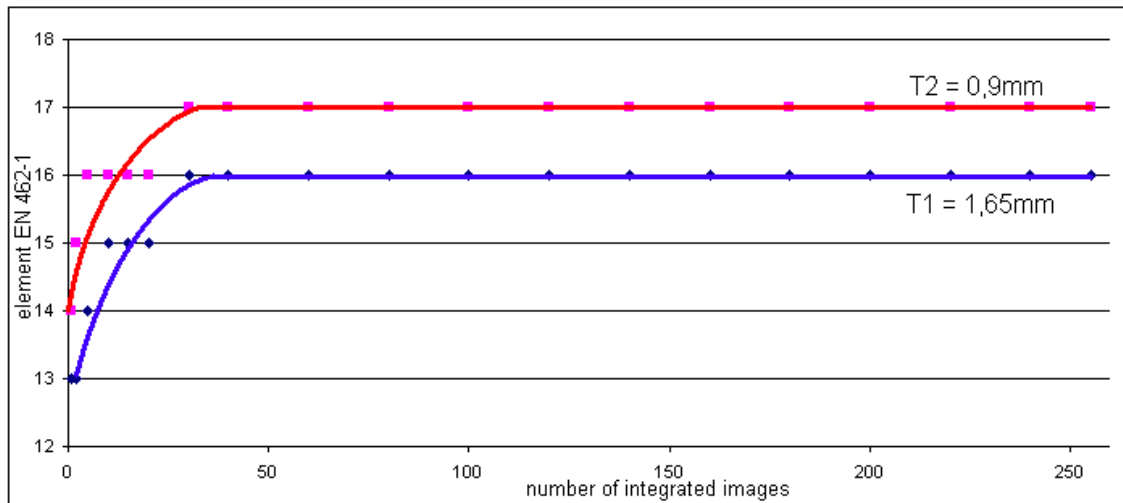
Figure 4.1 – Influence of the integration number to achieved image quality
